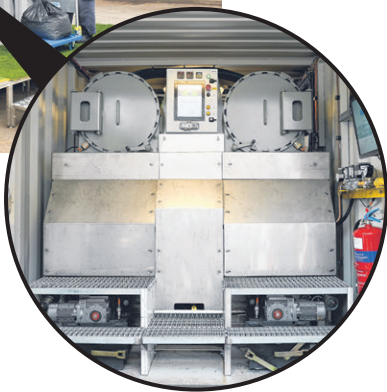
A worker from Gardens by the Bay wheeling a bag of waste to a compact gasification system housed in a 20-foot container.
